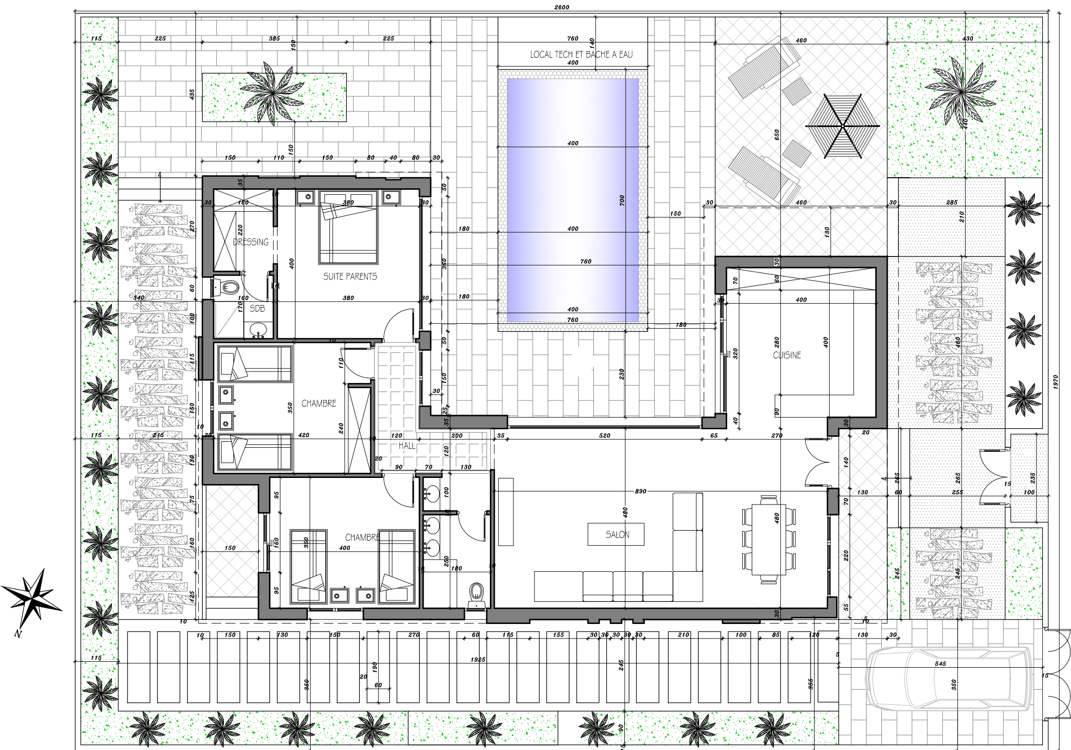
plan RDC sc dalle 172 m 2 sc habitable 146.3 m 2
