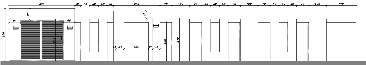
DETAIL CLOTURE
